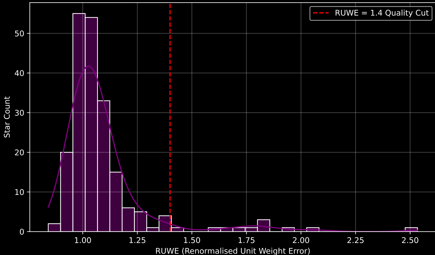
GALAH DR4 Field [51] RUWE Distribution (n= 206)
