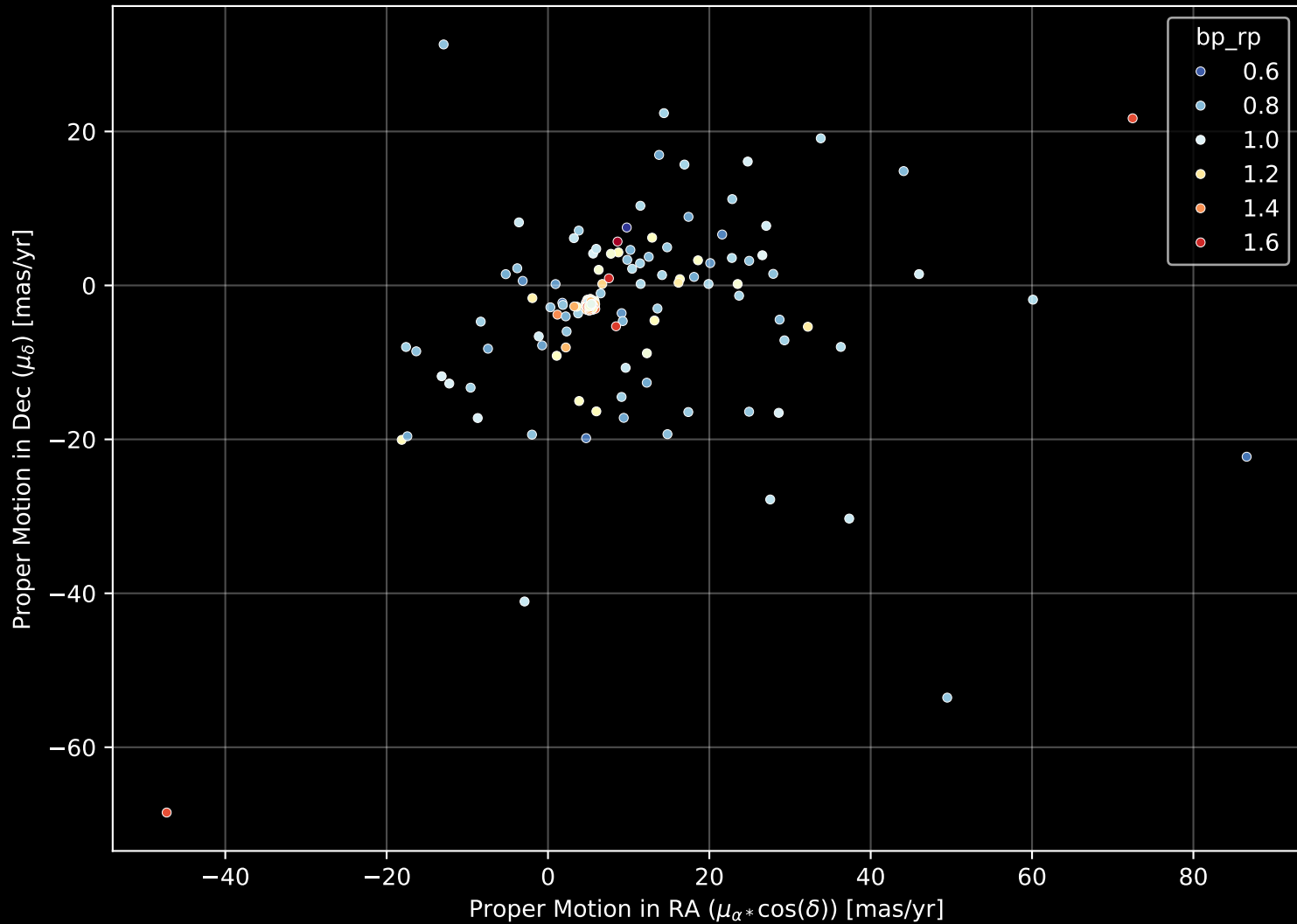
GALAH DR4 Field: [51] Proper Motion Diagram (n= 208)
