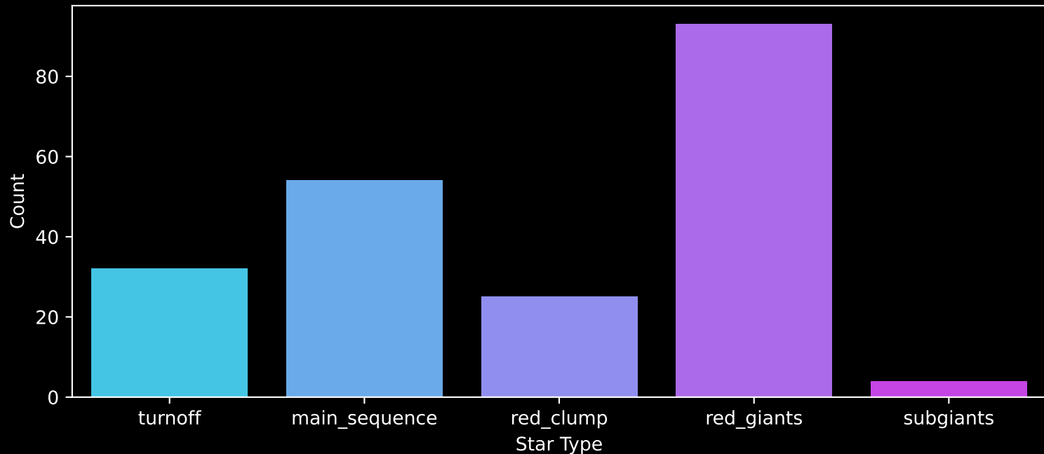
GALAH DR4 Field: [51] Count plot of Star Type
