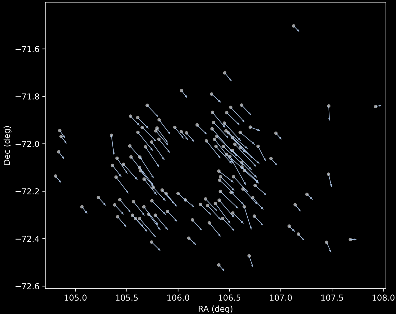
GALAH DR4 Cluster 1 Proper Motion Vectors (n=114)
